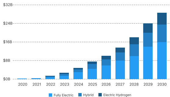
eVTOL Aircraft Market Size by Propulsion, 2020 – 2030 (USD Billion)
