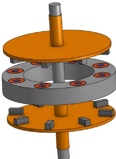
Maximum Air-Gap
