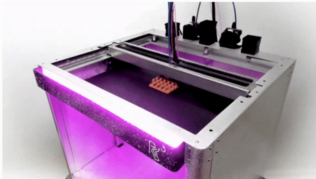
Never-before-seen footage of R3 Printer printing a custom-designed copper heat sink. R3 Printer is not yet on the market but is currently being tested by prospective customers as of Fall 2022
